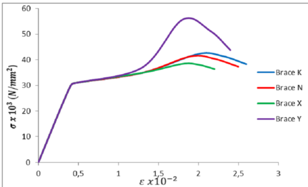
Fig. 3. Stress-strain Curve Relationship
